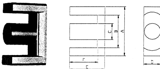
Product overview EER cores
