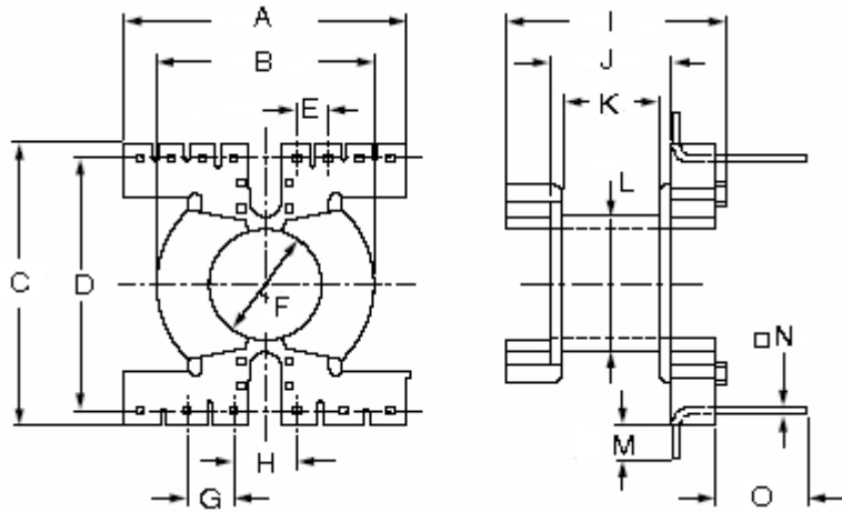
COILFORMER DIMENSIONS (mm)
