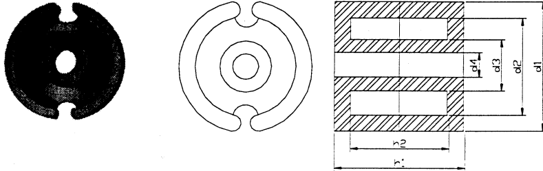
Product overview pot cores
